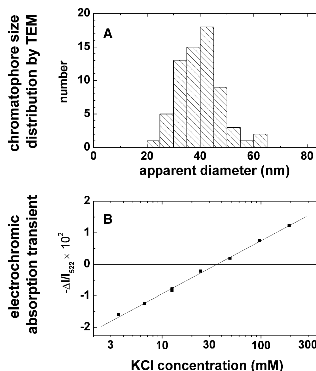
FIGURE 1 (A) Size distribution of \text{F}_1 -depleted chromatophores by transmission electron microscopy (TEM). Because of drying on the microscope grid the originally spherical particles appeared as flat disks (see text). (B) Absorption transients attributable to carotenoid bandshifts of electrochromic origin as function of the \text{K}^+ concentration in the suspending medium. These transients were caused by a diffusion potential that was generated by submitting chromatophores to a \text{K}^+ -concentration jump in the presence of the \text{K}^+ -ionophore valinomycin. \text{F}_1 -depleted chromatophores (940 \mu\text{M} bacteriochlorophyll) were preincubated with 45 mM KCl, 205 mM NaCl, 5 mM \text{MgCl}_2 , 20 mM glycylglycine-NaOH, pH 7.9. The final bacteriochlorophyll concentration in the samples was 12 \mu\text{M} .
